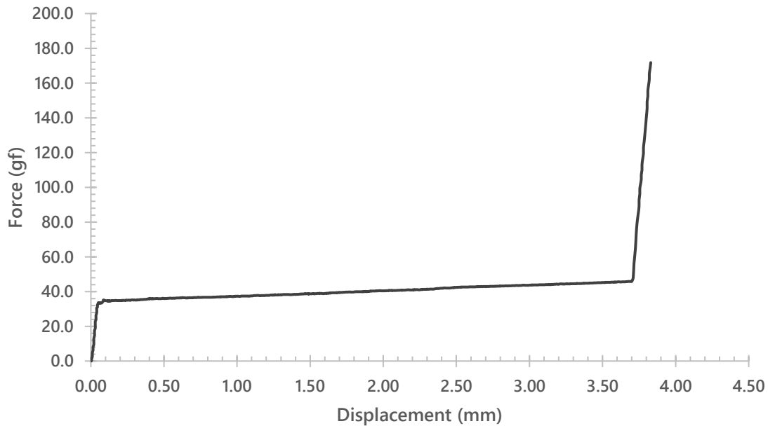
Keygeek T2 (45g) (Upstroke)
